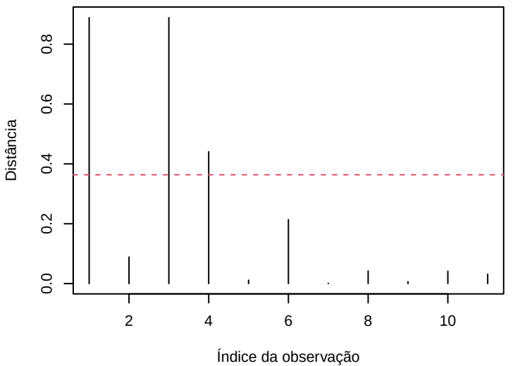
Cook's distance
