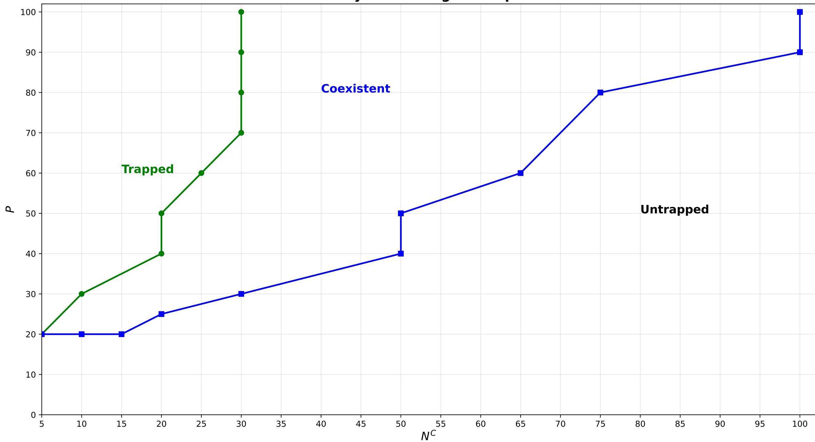
Dynamical-regime map
