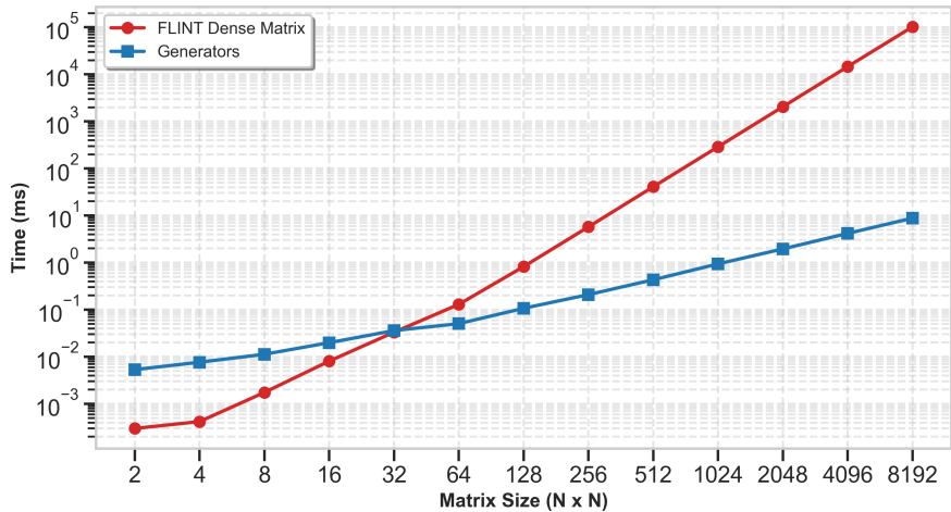
Multiplication Benchmark
