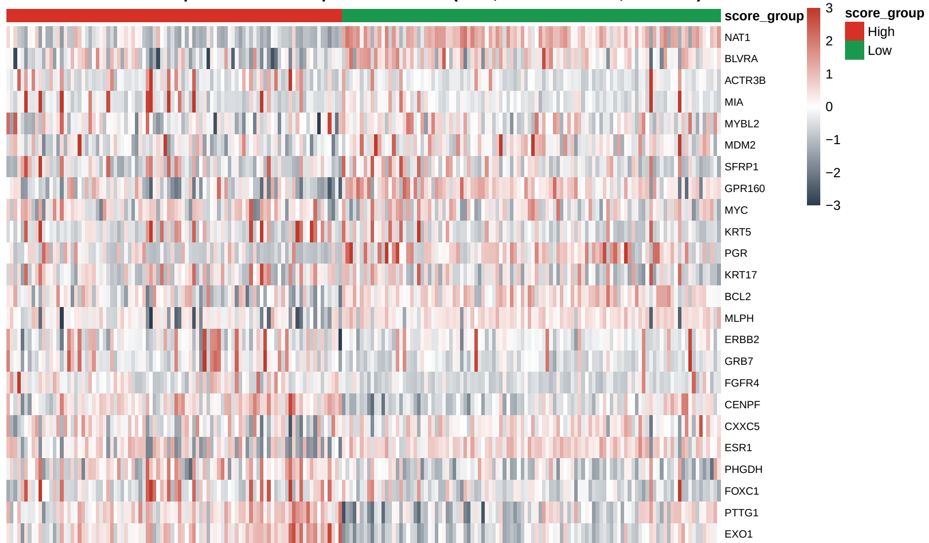
Core-PAM Gene Expression Heatmap — METABRIC (DSS, n=200 random, seed=42)
