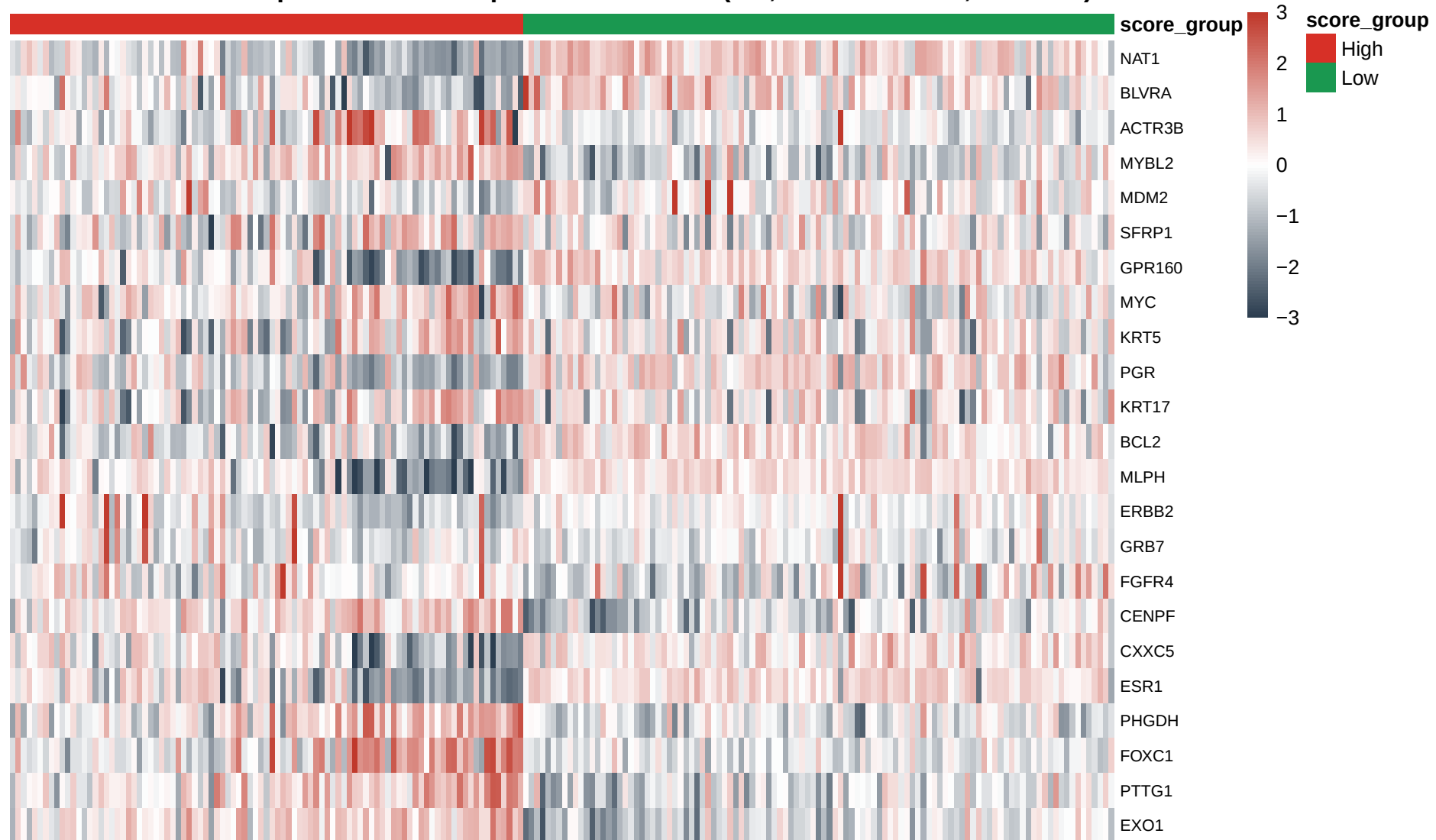
Core-PAM Gene Expression Heatmap — TCGA-BRCA (OS, n=200 random, seed=42)
