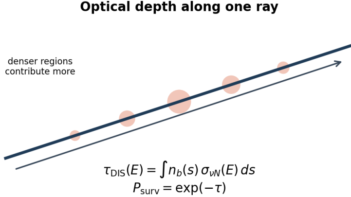
Figure 2: Optical depth and survival probability along a ray.
