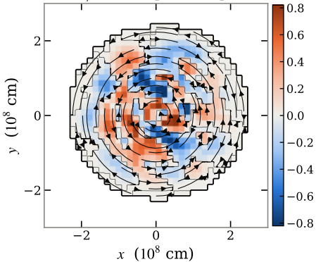
(a) B_\phi in the equatorial plane
