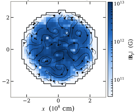
(b) \mathbf{B}_p in the meridional plane
