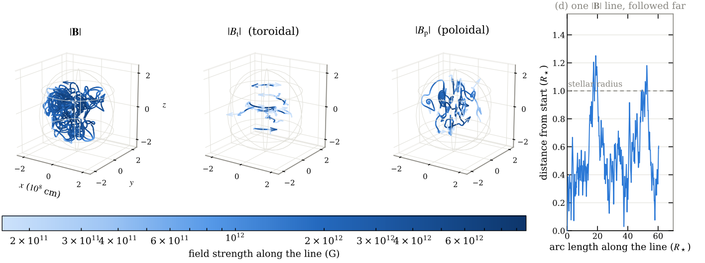
Fig. 5. Panels (a)-(c): field lines of the same three fields as Fig. 4, traced from a common set of starting points in the strong-field region, colored by the local field strength on a shared scale, with arrowheads giving the direction. The faint wireframe is the stellar surface. Each line is truncated at a fixed integration length, so its ends are a drawing choice and not a property of the field. Lines of the total and poloidal fields are tangled on scales short of the stellar radius; lines of the toroidal component are closed circles about the z axis by construction, so that panel shows where the toroidal field is strong rather than a structure the relaxation selected. Panel (d): one line of the total field followed to 60 stellar radii of arc, plotted as its distance from its own starting point. It ranges over the whole stellar volume without closing – the truncation in (a) hides this, and generic three-dimensional field lines do not close.
