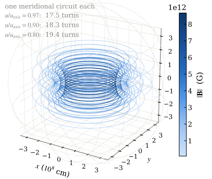
Fig. 3. Field lines of the same configuration in three dimensions, coloured by field strength, with the stellar surface as the faint wire-frame. Each line is drawn for exactly one meridional circuit, and the three are seeded at the flux levels labelled – all inside the closed region, u > 0.775 u_{\text{axis}} , so each lies on a torus contained in the star. Winding rises outward across that region. The lines do not close on themselves: the winding number is not an integer, so each circuit returns a line to its starting meridional plane at a different azimuth.
