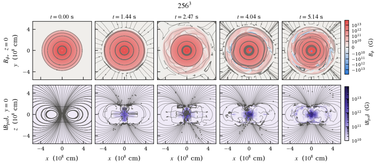
Figure 6: 256^3 , same layout, planes and colour scales as Fig. 1, at the corresponding instants.
