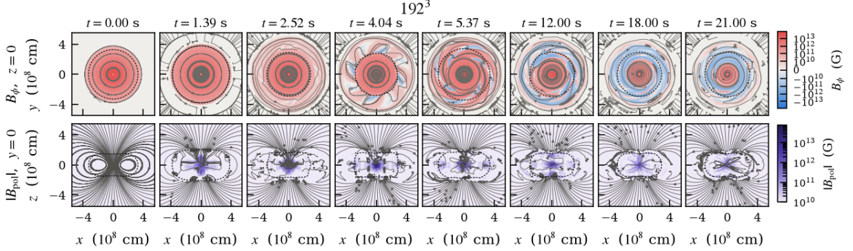
Figure 1: 192 3 . Top: equatorial cut z = 0 , where B_\varphi lies in the plane, so the streamlines of (B_x, B_y) are the toroidal field lines – circles while the star is axisymmetric, and their departure from circles is the instability. Colour is B_\varphi . Bottom: meridional cut y = 0 , where (B_x, B_z) is the poloidal field and the lines are its loops. Colour is |B_{\text{pol}}| . Both maps start at the same 10^{10} G, so the near-empty poloidal panel at t = 0 is the statement that the poloidal field is three decades below the toroidal one. Dashed: \rho = 10^6 \text{ g cm}^{-3} . Same scales as Fig. 6.
