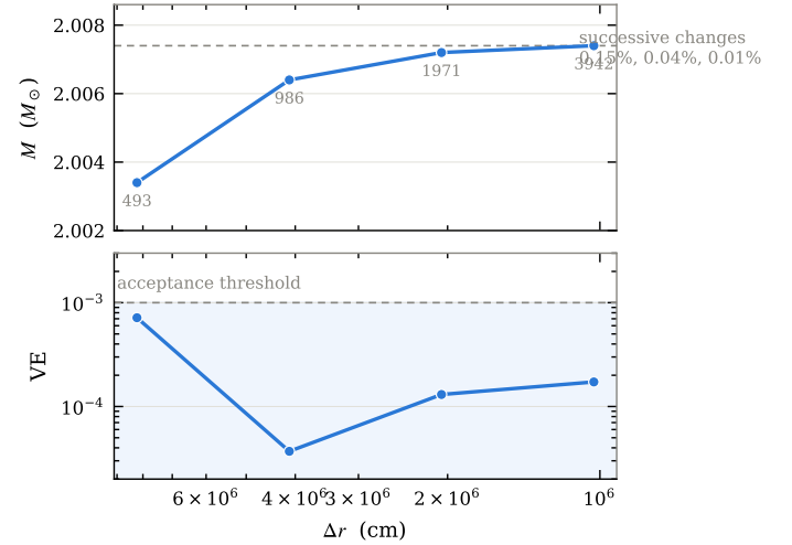
Fig. 4. Mesh convergence of the adopted configuration at fixed domain, labelled by radial resolution. Upper panel: the mass, converging monotonically to 2.007 M_\odot ; the dashed line is the finest value. Lower panel: the virial error, which stays inside the acceptance band (shaded) at every resolution without being monotonic.
