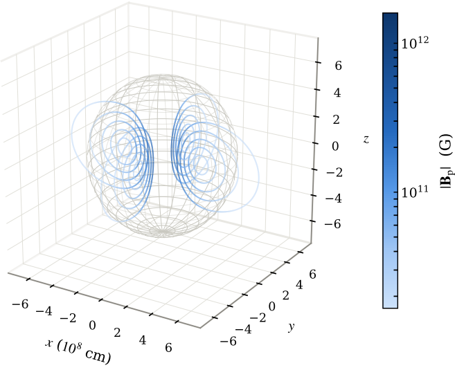
Fig. 2. The poloidal component alone, in three dimensions, coloured by |B_p| . A poloidal line stays in one meridional plane and is exactly a contour of the flux function there, so each is a planar closed loop about the O-point; loops are drawn at u/u_{\text{axis}} = 0.97, 0.90, 0.80, 0.68 and 0.55 , and repeated at four azimuths. The first three close inside the star and are the surfaces Fig. 3 winds its lines on; the last two cross the surface and close outside, where the density and hence B_\phi vanish and the field is purely poloidal. The wireframe is the stellar surface itself, prolate as a toroidal field makes it, not a sphere.
