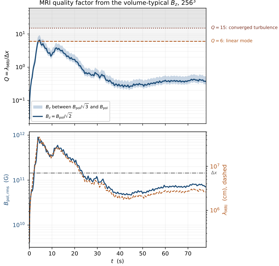
Figure 1: MRI quality factor at 256^3 . The band spans the three ways of splitting the poloidal energy between B_\varpi and B_z , from all of it vertical to isotropic; the spread is a factor 1.73, smaller than the effect being measured. Q peaks at 6.5 at t = 4.5 s — during the m = 1 disruption, when E_{\text{pol}} is at its largest — and decays to \simeq 0.4 thereafter. Q \geq 6 holds in 3% of the 210 samples under the central assumption, in none under the isotropic one. Q \geq 15 is reached under no assumption at any time. This figure alone uses the run extended to t = 78 s; everything else in the report is measured to t = 58.2 s. Data: investigations/mri_wavelength.py.
