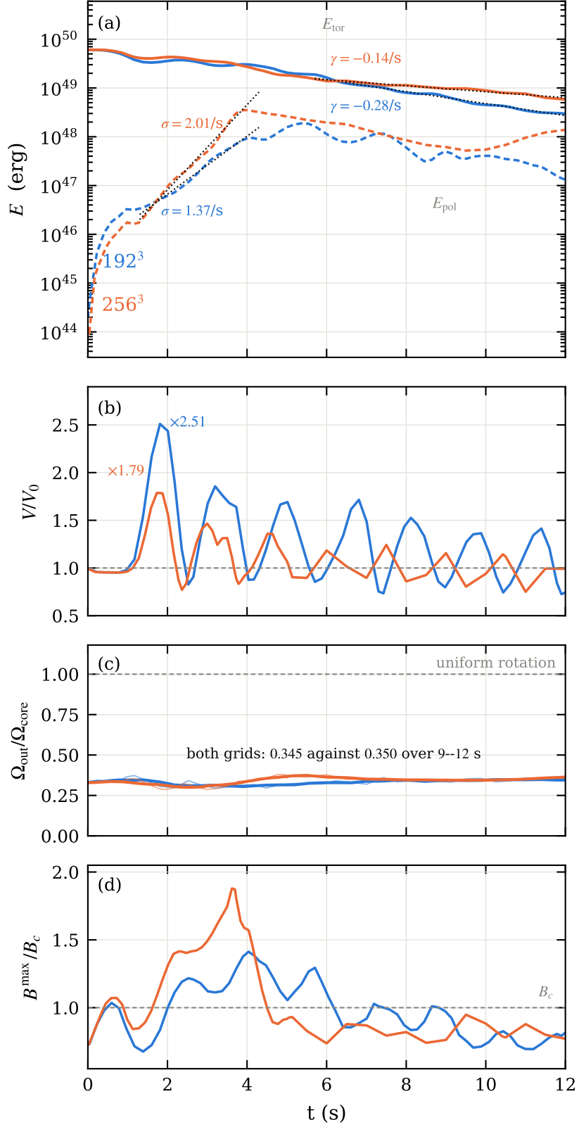
Figure 6: 192^3 against 256^3 over the full 12s. (a) Toroidal (solid) and poloidal (dashed) energy, with the fitted growth \sigma and decay \gamma . The two rates move in opposite directions with refinement. (b) V/V_0 : the first peak drops from 2.51 to 1.79, its excess over unity scaling as dx^{2.3} . (c) The differential rotation — neither grid approaches uniform rotation and the two agree to 1.4%. (d) Peak field against B_c ; above the Landau field for roughly half the run at both resolutions.
