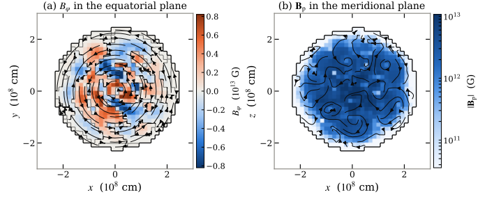
Fig. 4. The two components of seed 20's relaxed field, each in the plane in which it lies entirely, cropped to just outside the stellar surface. (a) B_\phi in the equatorial plane, signed, with its zero contour – the null surfaces separating oppositely circulating regions – and the in-plane streamlines of \mathbf{B}_t . Those are concentric circles by construction, since \mathbf{B}_t is azimuthal; what their arrows add is the sense of circulation, read directly rather than decoded from the colour, reversing wherever B_\phi does. (b) B_p in the meridional plane, as in-plane streamlines over its magnitude; there the streamline geometry is not fixed in advance and shows the poloidal topology. Both panels are masked to the stellar interior, outside which the field is at its numerical floor. Neither component is solenoidal by itself, which is why they are drawn this way rather than as three-dimensional field lines.
