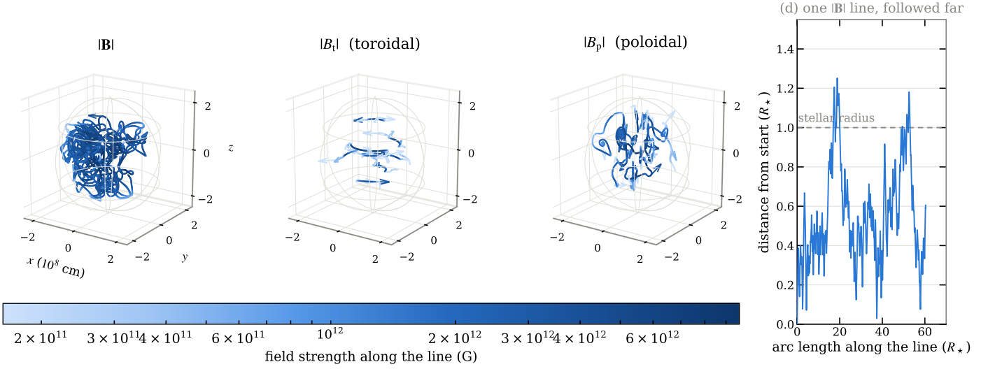
Fig. 5. Panels (a)-(c): field lines of the total field and of its toroidal and poloidal parts, traced from a common set of starting points in the strong-field region, colored by the local field strength on a shared scale, with arrowheads giving the direction. The faint wireframe is the stellar surface. Each line is truncated at a fixed integration length, so its ends are a drawing choice and not a property of the field. Lines of the total and poloidal fields are tangled on scales short of the stellar radius; lines of the toroidal component are closed circles about the z axis by construction, so that panel shows where the toroidal field is strong rather than a structure the relaxation selected. Panel (d): one line of the total field followed to 60 stellar radii of arc, plotted as its distance from its own starting point. It ranges over the whole stellar volume without closing – the truncation in (a) hides this, and generic three-dimensional field lines do not close.
