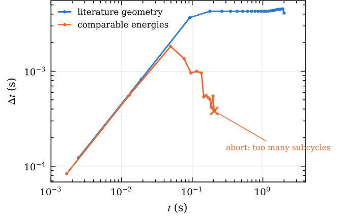
Figure 5. Time step against elapsed physical time for the two configurations, which differ only in poloidal amplitude on an otherwise identical star. Both ramp identically from the initial reduction. The literature geometry then holds a step of a few times 10^{-3} s and reaches the target time; the comparable-energy configuration peaks at t \simeq 0.05 s and loses the step in plateaus until the subcycle limit ends the run at t = 0.205 s. The pair is asymmetric by construction — only one of the two is ambient-limited — so the figure shows the constraint of Section 5, not a difference in stability.
