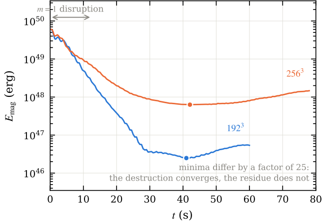
Figure 4. Magnetic energy of the star against time on both meshes. The ordered field loses most of its energy over the first several seconds and the decay is robust: the two meshes agree on it. Where they do not agree is the level the field settles to, the minima differing by a factor of 25, after which the energy rises again on both. We show both meshes rather than one so that the residue is not mistaken for a measurement; growth rates and residues are reported as resolution-limited throughout (Section 7).
