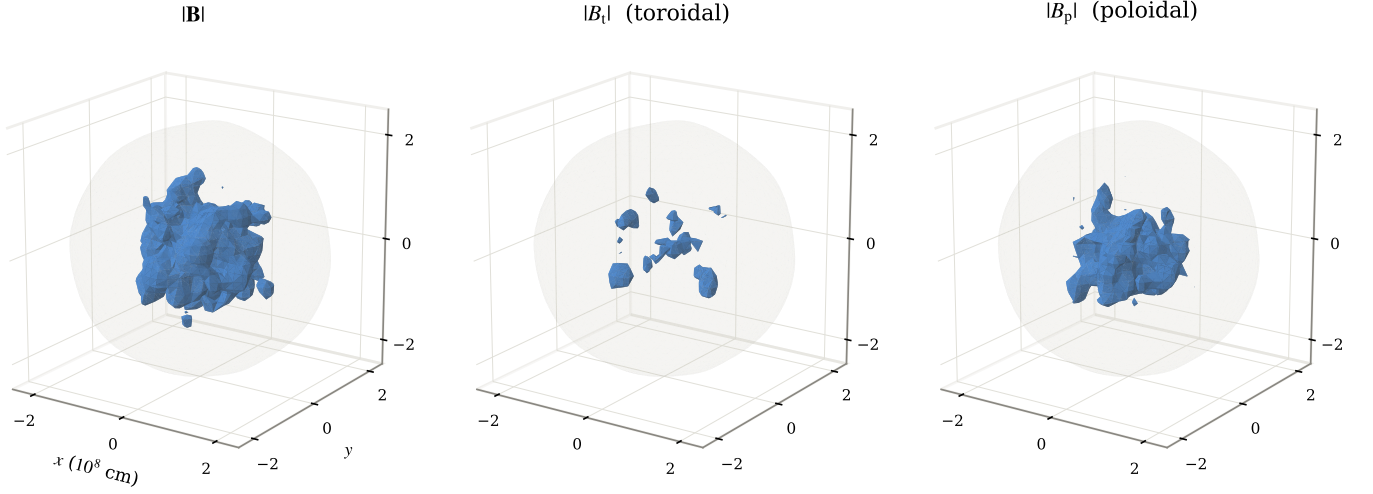
Fig. 5. Isosurfaces of the same three fields as Fig. 4, all at the same level, 5.96 \times 10^{12} G (the 90th percentile of |\mathbf{B}| inside the star), so that the enclosed volumes are directly comparable. The translucent envelope is the stellar surface. The strong-poloidal region is a single connected structure; the strong-toroidal region is fragmented.
