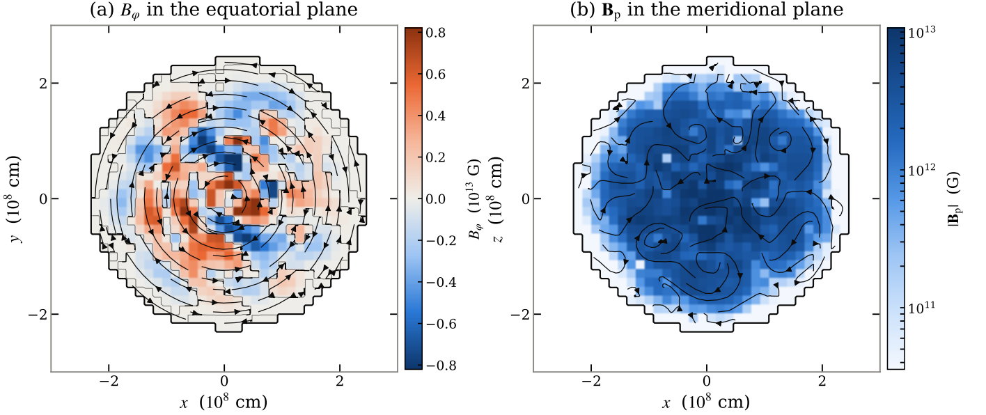
Fig. 6. The two components of seed 20's relaxed field, each in the plane in which it lies entirely, cropped to just outside the stellar surface. (a) B_\phi in the equatorial plane, signed, with its zero contour – the null surfaces separating oppositely circulating regions – and the in-plane streamlines of \mathbf{B}_t . Those are concentric circles by construction, since \mathbf{B}_t is azimuthal; what their arrows add is the sense of circulation, read directly rather than decoded from the colour, reversing wherever B_\phi does. (b) B_p in the meridional plane, as in-plane streamlines over its magnitude; there the streamline geometry is not fixed in advance and shows the poloidal topology. Both panels are masked to the stellar interior, outside which the field is at its numerical floor. Neither component is solenoidal by itself, which is why they are drawn this way rather than as three-dimensional field lines.
