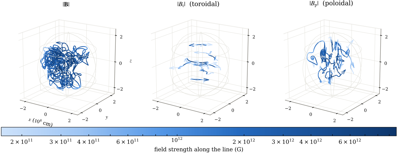
Fig. 5. Field lines of the total field and of its toroidal and poloidal parts, traced from a common set of starting points in the strong-field region, colored by the local field strength on a shared scale, with arrowheads giving the direction. The faint wireframe is the stellar surface. Each line is truncated at a fixed integration length, so its ends are a drawing choice and not a property of the field. Lines of the total and poloidal fields are tangled on scales short of the stellar radius; lines of the toroidal component are closed circles about the z axis by construction, so that panel shows where the toroidal field is strong rather than a structure the relaxation selected.
