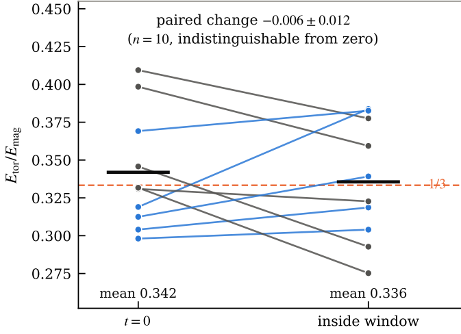
Fig. 4. Toroidal fraction at t = 0 and averaged inside the validity window, paired per seed, for the batch of ten. Blue lines increase, gray lines decrease; heavy bars are the ensemble means, and the dashed line is the isotropic value 1/3 . Individual seeds move; the ensemble mean does not.
