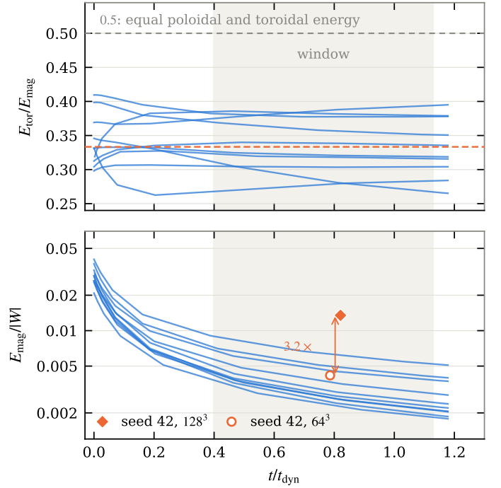
Fig. 3. Evolution of the ten seeds of one batch at 64^3 , with the validity window shaded. Upper panel: toroidal fraction, which stays within a narrow band well below 0.5 throughout, with the isotropic value 1/3 marked. Lower panel: magnetic energy, which falls by about an order of magnitude, and the same seed measured at both resolutions – the 128^3 run retains 3.2 times more field energy at the same time, so this decay is resolution-limited.
