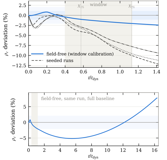
Fig. 2. Central density relative to its initial value. Upper panel: the field-free calibration run (thick) and the three extended seeded runs (thin), with the \pm 1\% and \pm 2\% bands, the crossings X_{1\%} = 0.573 and X_{2\%} = 1.128 that define the upper bound, and the resulting window shaded. The seeded runs leave the \pm 2\% band well before the window closes. Lower panel: the same field-free run over its full baseline – the drift never settles.
