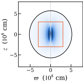
(a) whole star
