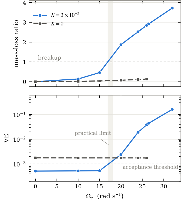
Fig. 4. Termination of the rotating sequence with and without a toroidal field, at \rho_c = 10^{12} \text{ g cm}^{-3} on an identical mesh. Upper panel: equatorial mass-loss ratio, which reaches unity at breakup and is unphysical beyond it. Lower panel: virial error, with the 10^{-3} acceptance threshold. With the field present both diagnostics fail together in the shaded interval, \Omega_c \approx 17\text{--}18 \text{ rad s}^{-1} , well before the field-free sequence shows any sign of terminating. The field-free point at \Omega_c = 26.5 \text{ rad s}^{-1} , where the solver jumps to a spurious branch, is omitted.
