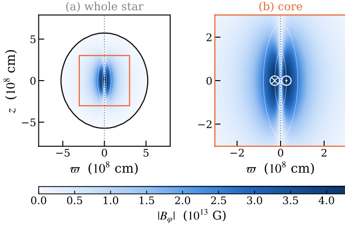
Fig. 3. Meridional cut of the M = 2.007 M_{\odot} configuration ( \rho_c = 10^9 \text{ g cm}^{-3} , K = 3.245 \times 10^{-3} , m = 1 , no rotation), colored by the toroidal field strength. Panel (a) is the whole star, with the stellar surface as the heavy contour; panel (b) is the boxed core region. Thin white curves are the \rho = 0.5 \rho_c and \rho = 0.1 \rho_c surfaces. The field is purely azimuthal: in this plane it points out of the page on one side of the axis and into it on the other, as marked at the field maximum. Both panels share the color scale.
