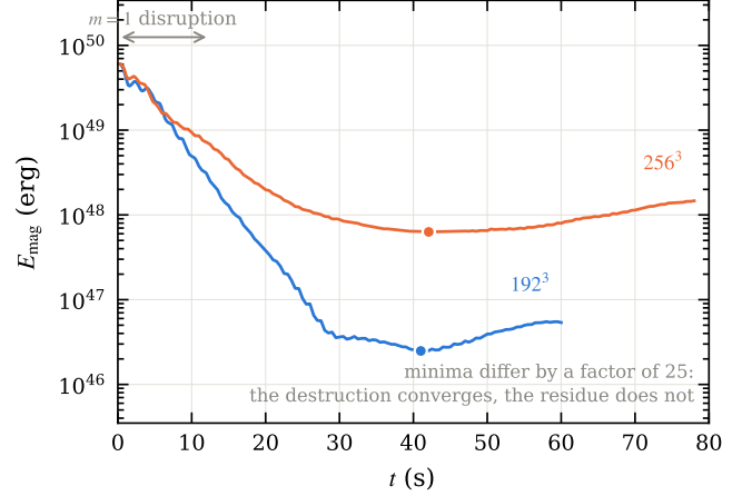
Figure 4. Magnetic energy of the star against time on both meshes. The ordered field is destroyed over the first several seconds and the decay is robust: the two meshes agree on it. Where they do not agree is the level the field settles to, the minima differing by a factor of 25, after which the energy rises again on both. We show both meshes rather than one so that the residue is not mistaken for a measurement; growth rates and residues are reported as resolution-limited throughout (Section 7).
