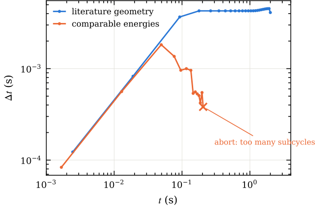
Figure 5. Time step against elapsed physical time for the two configurations, which differ only in poloidal amplitude on an otherwise identical star. Both ramp identically from the initial reduction. The literature geometry then holds a step of a few times 10^{-3} s and reaches the target time; the comparable-energy configuration peaks at t \simeq 0.05 s and loses the step in plateaus until the subcycle limit ends the run at t = 0.205 s. The pair is asymmetric by construction — only one of the two is ambient-limited — so the figure shows the constraint of Section 5, not a difference in stability.
