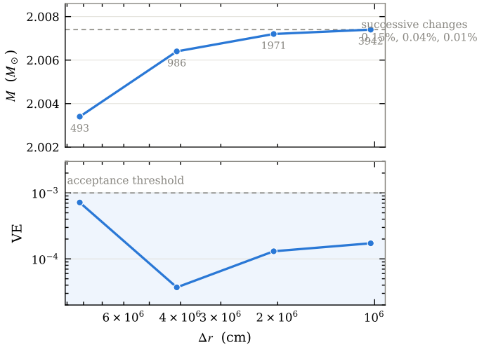
Fig. 4. Mesh convergence of the adopted configuration at fixed domain, labelled by radial resolution. Upper panel: the mass, converging monotonically to 2.007 M_\odot ; the dashed line is the finest value. Lower panel: the virial error, which stays inside the acceptance band (shaded) at every resolution without being monotonic.
