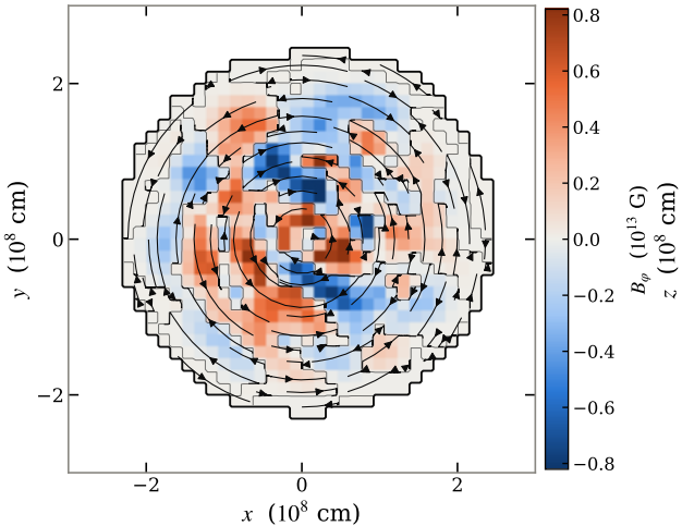
(a) B_\phi in the equatorial plane
