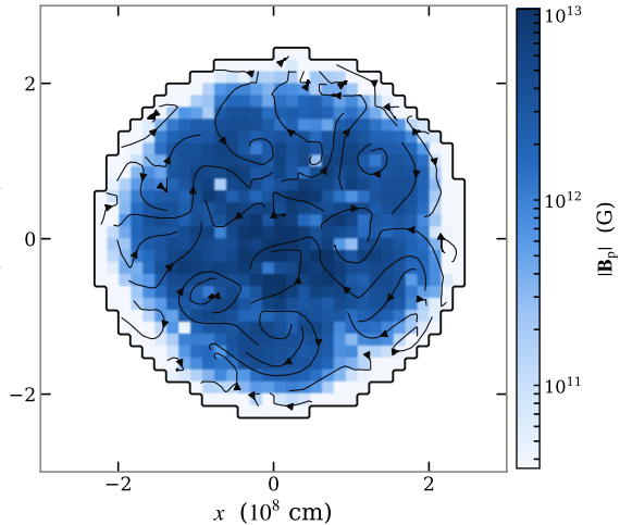
(b) \mathbf{B}_p in the meridional plane
