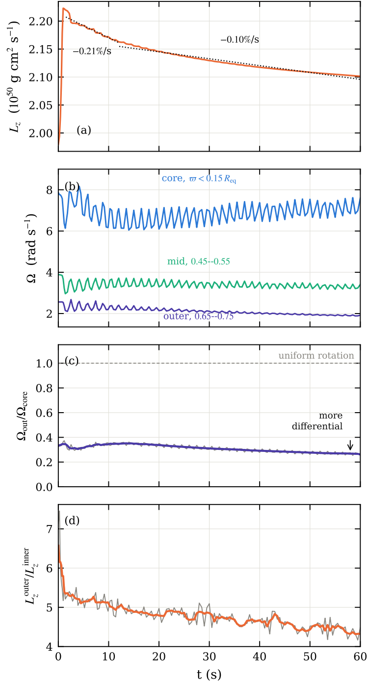
Figure 1: 192^3 over the full 60 s. (a) L_z of the star, with the two braking rates fitted; the 12% rise in the first second is the initial transient settling. (b) \Omega mass-weighted in three cylindrical shells, all chosen to stay inside the star at every phase of the 1.5 s pulsation. (c) the differential rotation itself; uniform rotation would be 1 and the star moves away from it. (d) L_z of the outer half of the mass over that of the inner half — split by mass rather than radius, with the dividing radius recomputed at every snapshot, because a shell at fixed \varpi would measure the pulsation instead of the transport. In (c) and (d) a running mean over one pulsation period is drawn over the raw curve; the ripple is the pulsation and aliases badly against coarse sampling.
