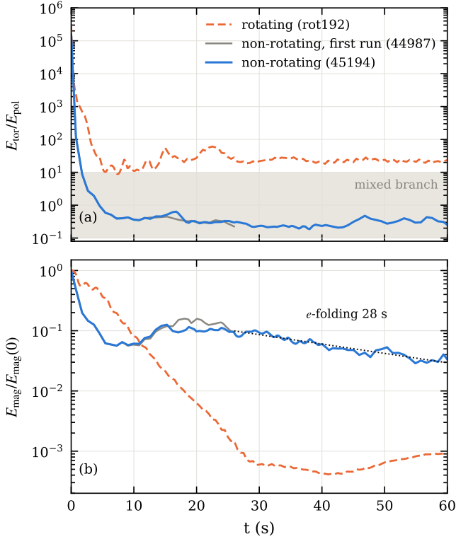
Figure 6. Field evolution with and without rotation, both at 192^3 . (a) E_{\text{tor}}/E_{\text{pol}} ; shading marks the comparable band of criterion (iii). Without rotation the ratio falls below unity at t \approx 4 s and stays between 0.19 and 0.64 to t = 60 s; with rotation it stays between 12 and 61 after t = 12 s. (b) Magnetic energy relative to its initial value. Without rotation it falls to 6% by t = 5 s, recovers to about 10%, and from t = 26 s decays with an e -folding time of 28 s (dotted) to 3.4% at t = 60 s; the rotating run retains 0.09%. The grey curve is the first non-rotating run, without ambient replenishment, which stalls at t = 26 s.
