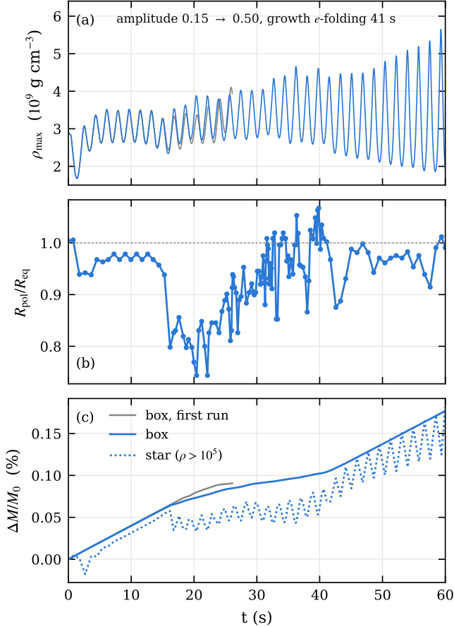
Figure 7. The non-rotating star. (a) Maximum density: a radial pulsation of period 1.77 s whose relative amplitude grows from 0.15 to 0.50 between t = 5 and 60 s. (b) Ratio of polar to equatorial radius, which follows the phase of the pulsation rather than the field. (c) Mass in the domain and in the star ( \rho > 10^5 \text{ g cm}^{-3} ) relative to t = 0 ; both rise by 0.18% as ambient material enters through the replenished boundary.
