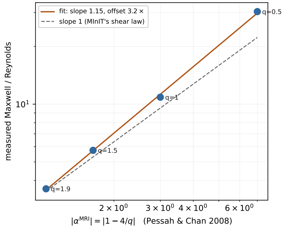
(b) MInIT's shear law against our data
