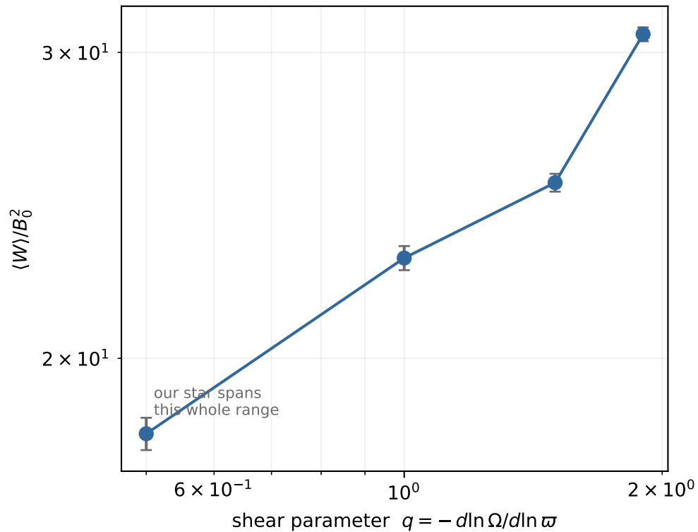
(a) Transport rises with shear, \propto q^{0.37}
