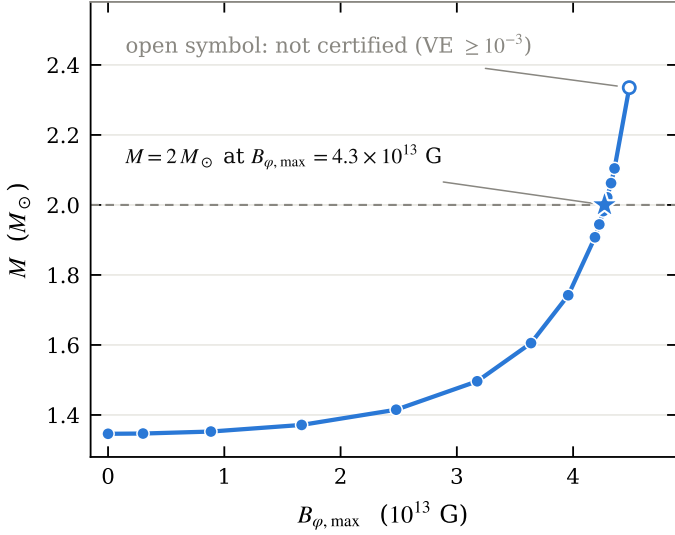
Fig. 2. Equilibrium mass along the toroidal sequence at \rho_c = 10^9 \text{ g cm}^{-3} ( m = 1 , no rotation), obtained by continuation from the field-free configuration. Filled symbols are certified ( \text{VE} < 10^{-3} ); the star marks the interpolated 2 M_{\odot} crossing.
