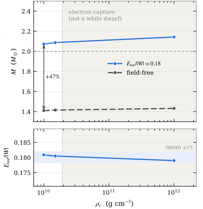
Fig. 1. Equilibrium mass with and without a purely toroidal field ( m = 1 , K = 3 \times 10^{-3} , no rotation) as a function of central density (upper panel), and the dimensionless field strength of the magnetized sequence (lower panel). The shaded region lies above the inverse-beta-decay threshold for \mu_e = 2 ( 1.94 \times 10^{10} \text{ g cm}^{-3} , the conservative ^{16}\text{O} value of Boshkayev et al. 2013), where the cold constant- \mu_e equation of state no longer describes a white dwarf; the \rho_c = 10^{12} configuration is shown for reference only. The band in the lower panel is the mean of the three measurements \pm 1\% .
