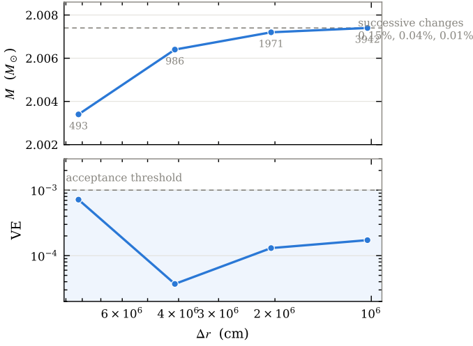
Fig. 2. Mesh convergence of the adopted configuration at fixed domain, labelled by radial resolution. Upper panel: the mass, converging monotonically to 2.007 M_\odot ; the dashed line is the finest value. Lower panel: the virial error, which stays inside the acceptance band (shaded) at every resolution without being monotonic.
