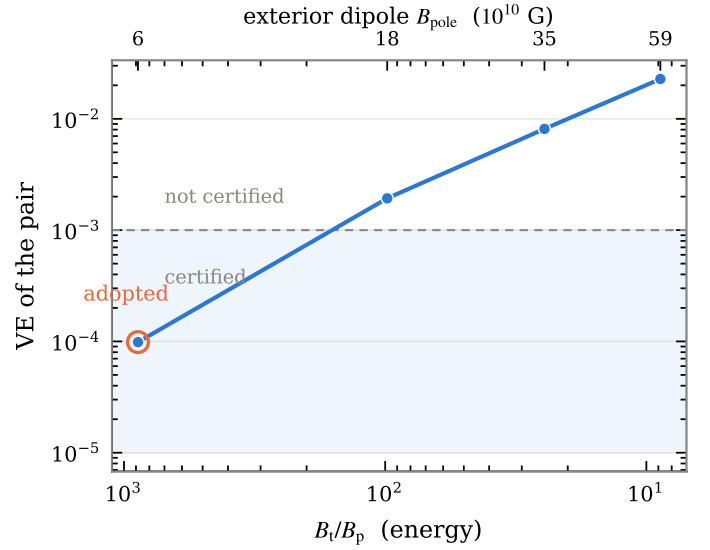
Fig. 3. The cost of the poloidal component. Moving left to right, the imposed poloidal amplitude rises, the field becomes less toroidal-dominated, and the exterior dipole (upper axis) grows; the virial error of the pair rises with it and leaves the certified band (shaded). The circled point is the configuration of Table 1.
