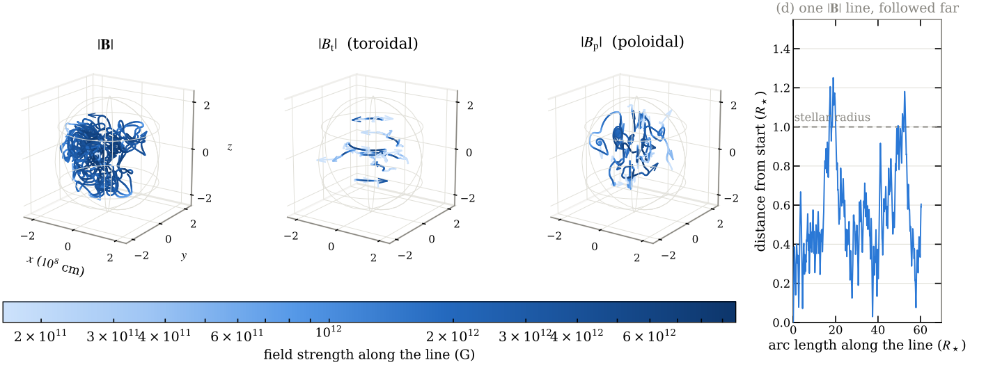
Fig. 4. Panels (a)-(c): field lines of the total field and of its toroidal and poloidal parts, traced from a common set of starting points in the strong-field region, colored by the local field strength on a shared scale, with arrowheads giving the direction. The faint wireframe is the stellar surface. Each line is truncated at a fixed integration length, so its ends are a drawing choice and not a property of the field. Lines of the total and poloidal fields are tangled on scales short of the stellar radius; lines of the toroidal component are closed circles about the z axis by construction, so that panel shows where the toroidal field is strong rather than a structure the relaxation selected. Panel (d): one line of the total field followed to 60 stellar radii of arc, plotted as its distance from its own starting point. It ranges over the whole stellar volume without closing – the truncation in (a) hides this, and generic three-dimensional field lines do not close.
