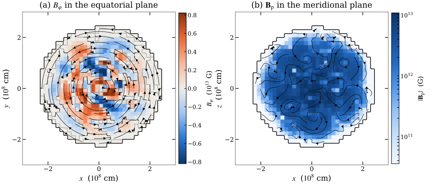
Fig. 5. The two components of seed 20's relaxed field, each in the plane in which it lies entirely, cropped to just outside the stellar surface. (a) B_\phi in the equatorial plane, signed, with its zero contour – the null surfaces separating oppositely circulating regions – and the in-plane streamlines of \mathbf{B}_t . Those are concentric circles by construction, since \mathbf{B}_t is azimuthal; what their arrows add is the sense of circulation, read directly rather than decoded from the colour, reversing wherever B_\phi does. (b) \mathbf{B}_p in the meridional plane, as in-plane streamlines over its magnitude; there the streamline geometry is not fixed in advance and shows the poloidal topology. Both panels are masked to the stellar interior, outside which the field is at its numerical floor. Neither component is solenoidal by itself, which is why they are drawn this way rather than as three-dimensional field lines.
