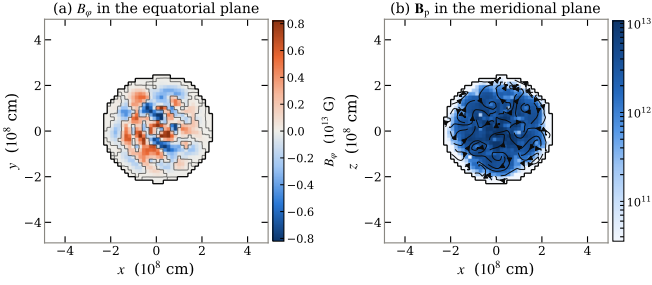
Fig. 5. The two components of seed 20's relaxed field, each in the plane in which it lies entirely. (a) B_\phi in the equatorial plane, signed, with its zero contour – the null surfaces separating oppositely circulating regions. (b) B_p in the meridional plane, as in-plane streamlines over its magnitude. Both are masked to the stellar interior, outside which the field is at its numerical floor. Neither component is solenoidal by itself, which is why they are drawn this way rather than as three-dimensional field lines.
