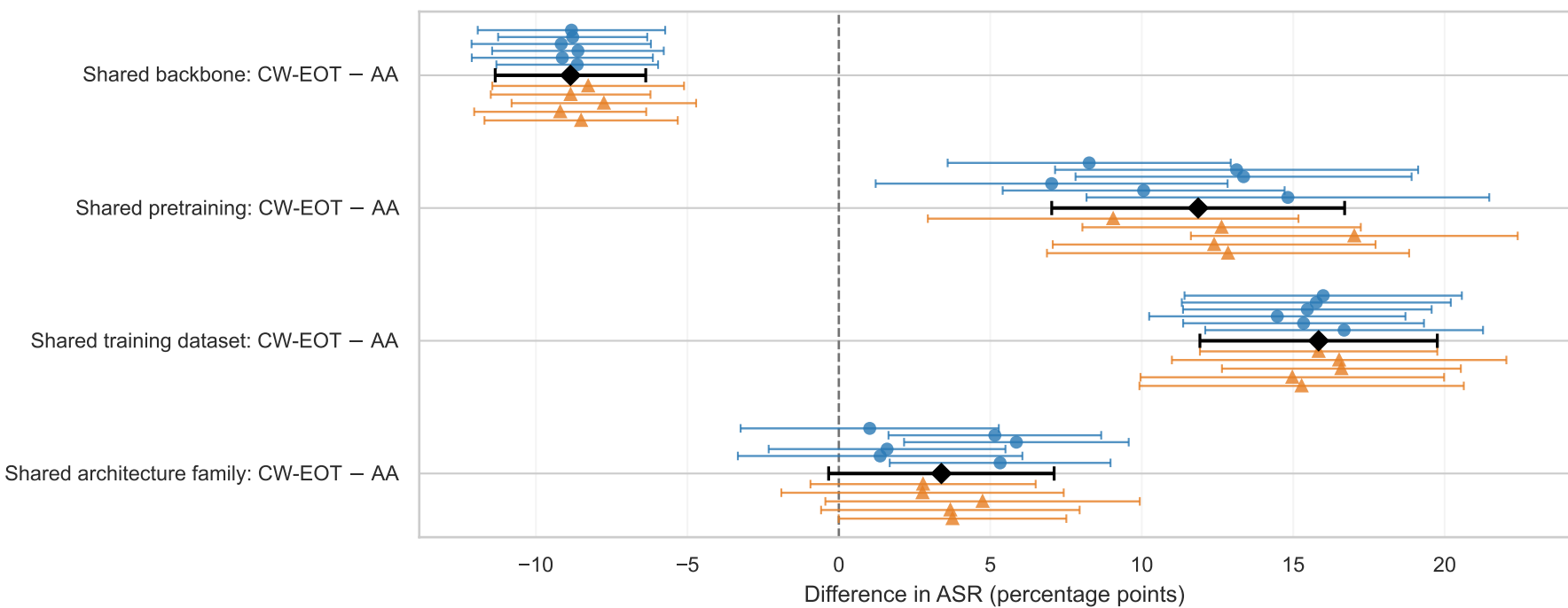
Overall attack contrast: CW-EOT – AA
