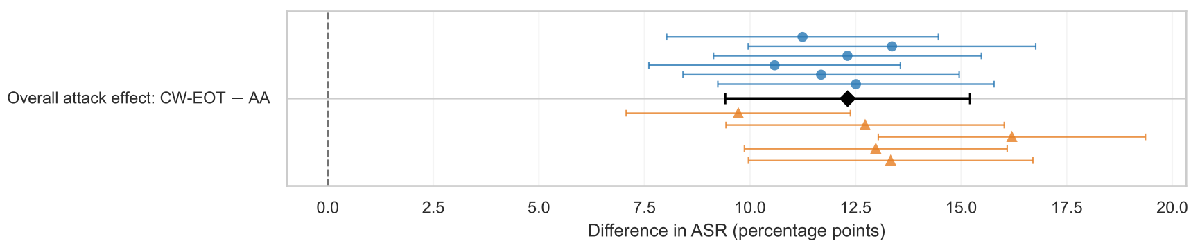
Overall attack contrast: CW-EOT – AA
