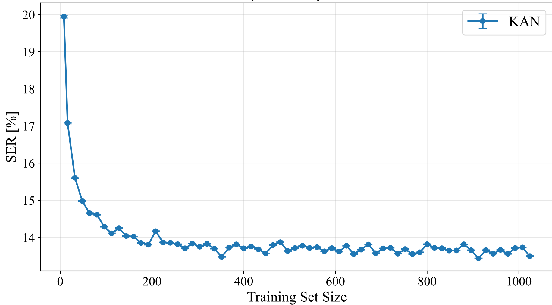
Sample Efficiency - 4CSK
