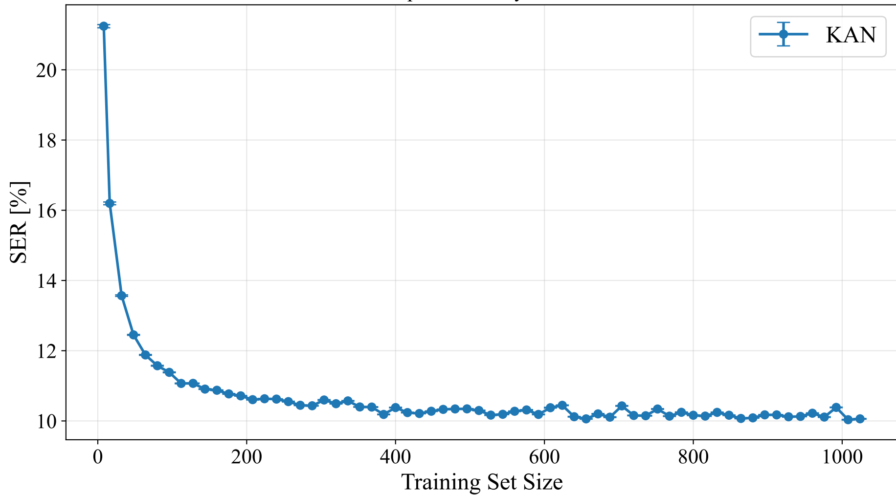
Sample Efficiency - 8CSK
