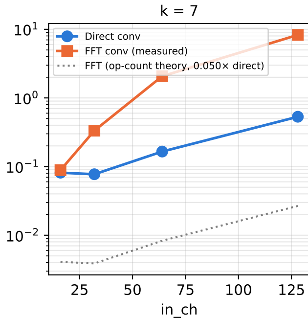
RTX 4060 Laptop (local): FFT vs. direct convolution (batch=1, res=64)
