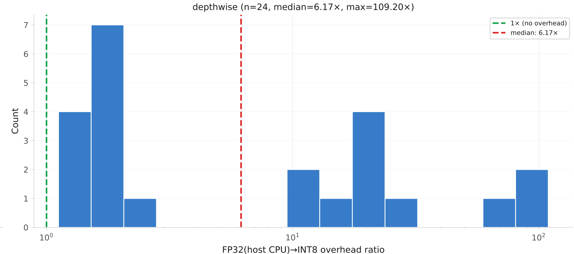
RTX 4060 Laptop (local): H4 — FP32→INT8 overhead distribution, host CPU, split by groups_mode
