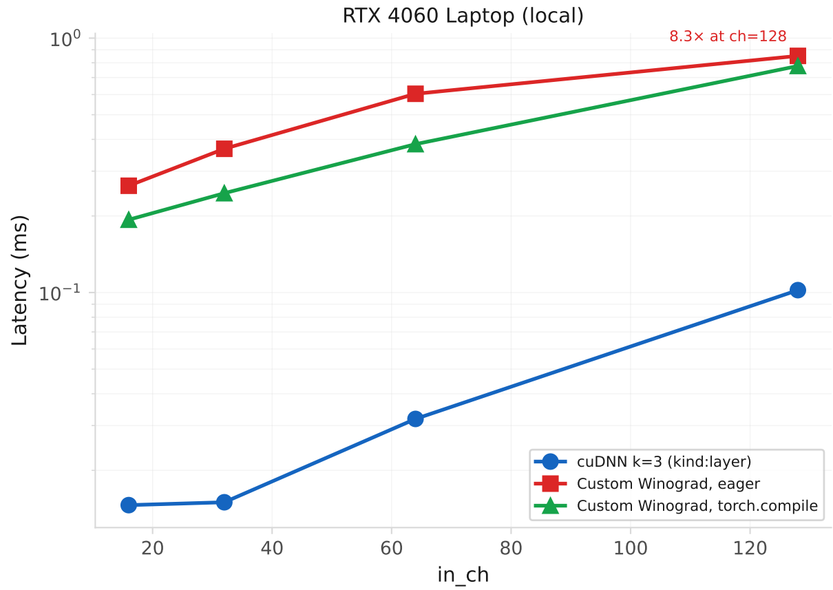
Custom Winograd F(2×2,3×3) vs. cuDNN's k=3 algorithm choice (batch=1, res=64)
