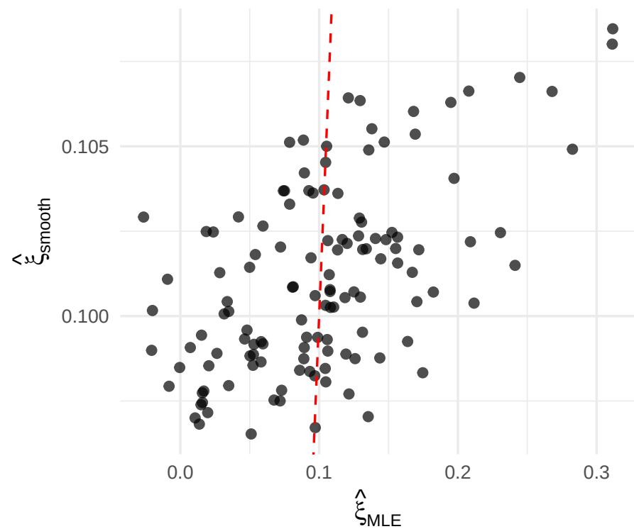
\xi (shape)
