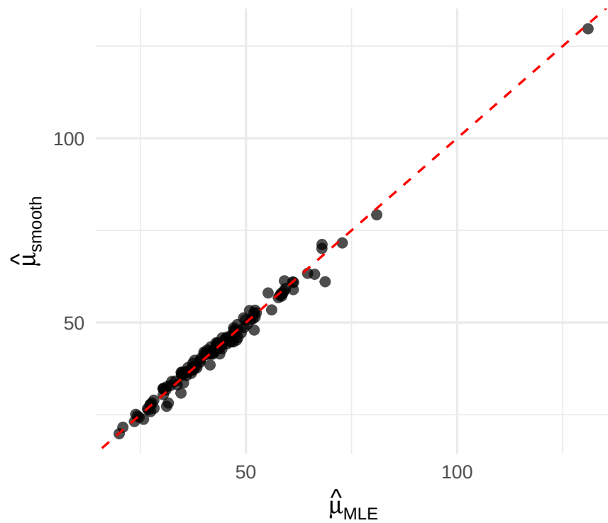
\mu (location)
