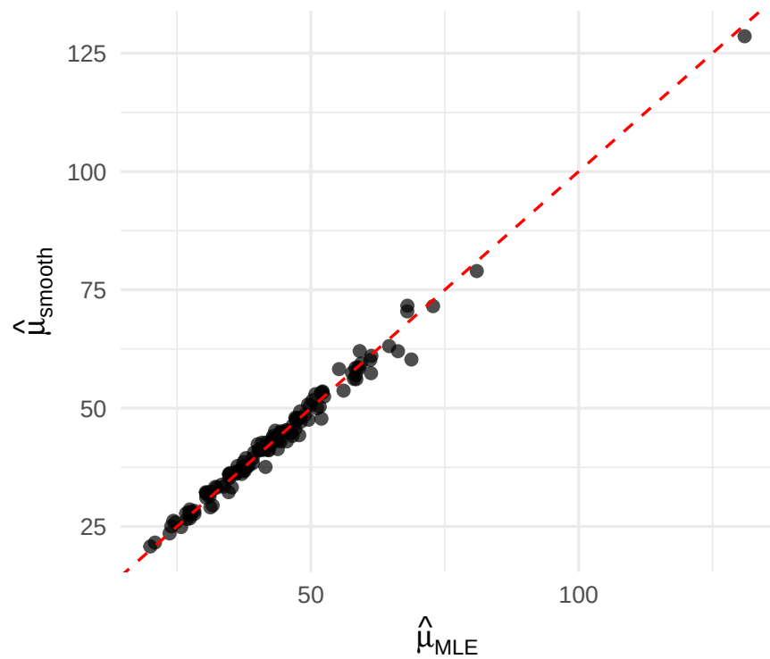
\mu (location)
