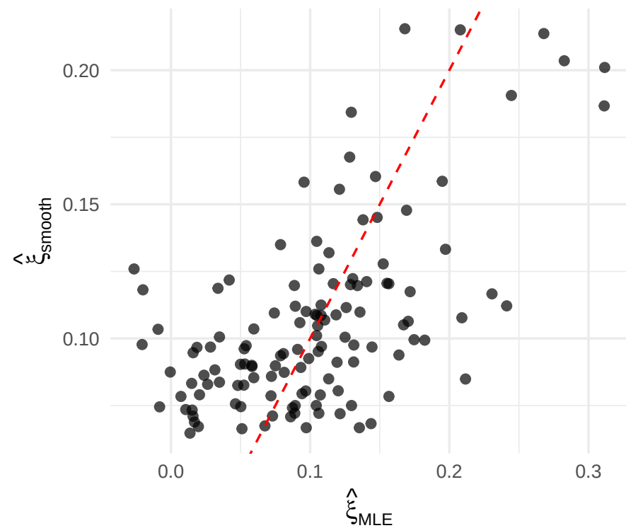
\xi (shape)
