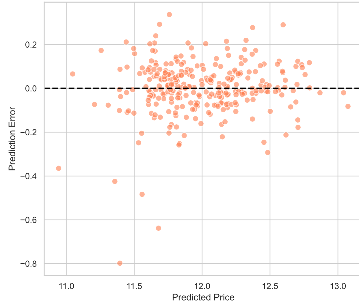
LassoCV: Residuals Plot
