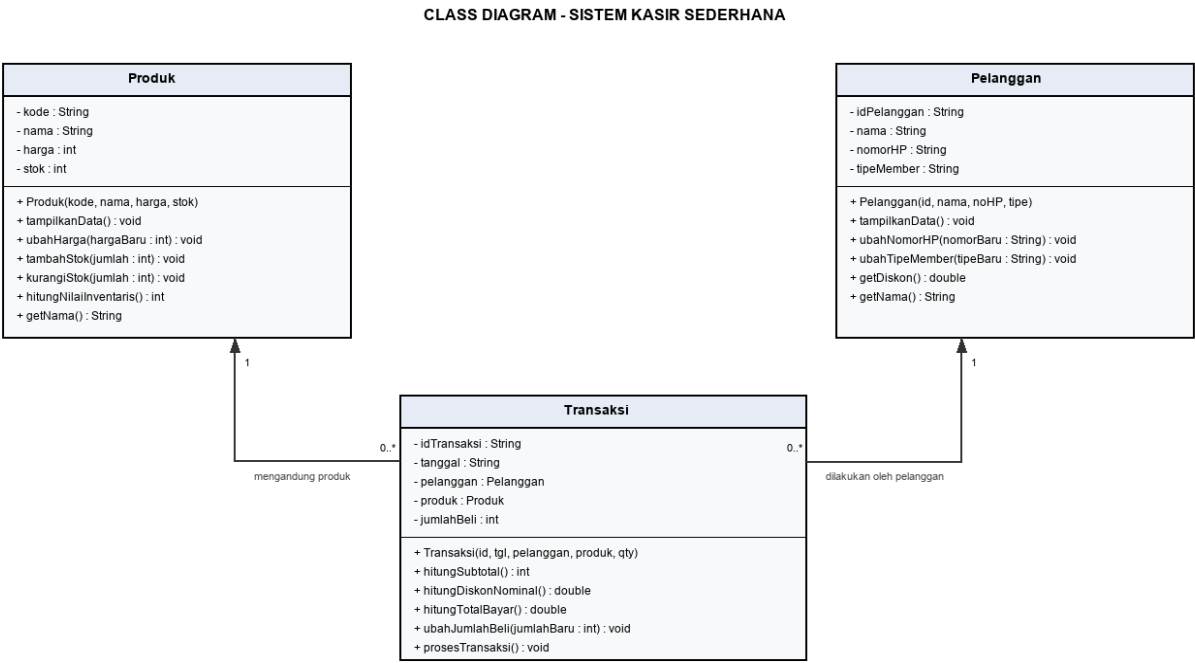
Gambar 1. UML Class Diagram Relasi Objek Kasir
