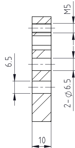
SECTION A
