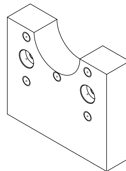
ISOMETRIC VIEW 1 : 2
