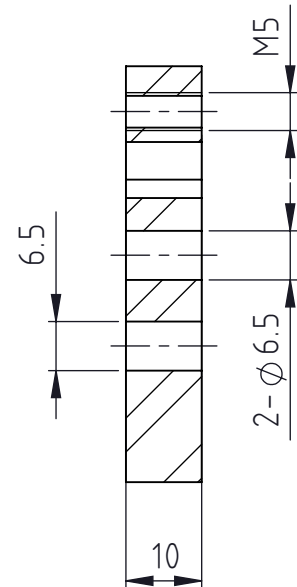
SECTION A
