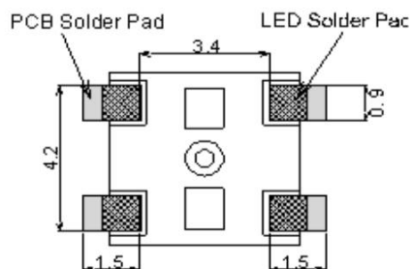
Solder Pad
