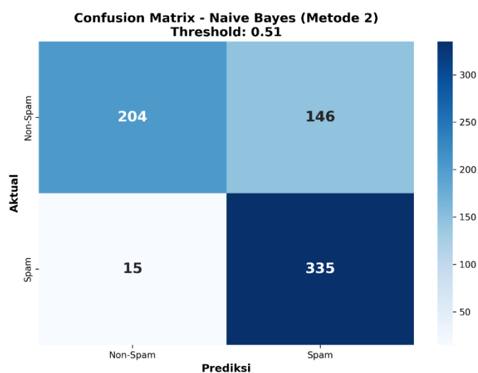
Gambar IV. 6 Confusion matrix Complement Naive Bayes Metode 2
