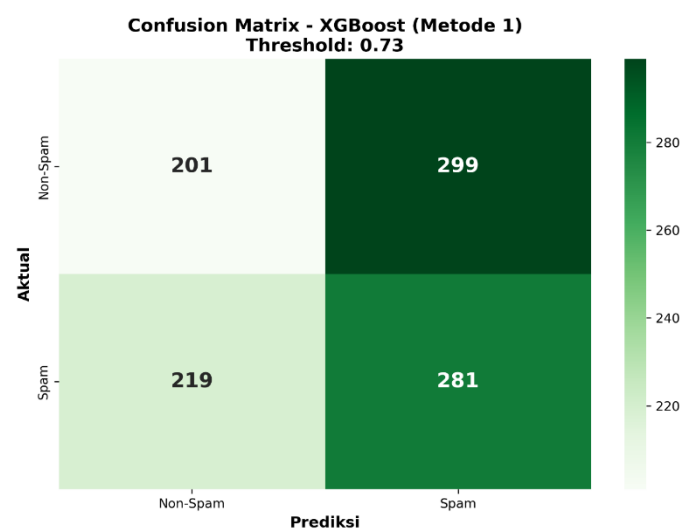
Gambar IV. 4 Confusion matrix XGBoost Metode 1
