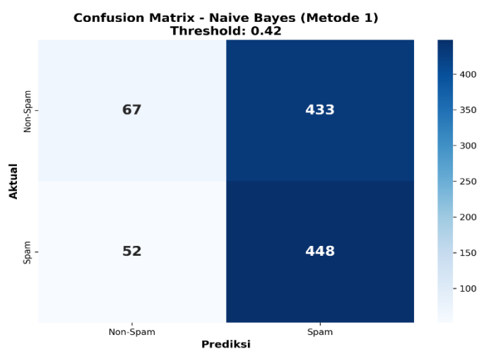
Gambar IV. 3 Confusion matrix Complement Naive Bayes Metode 1
