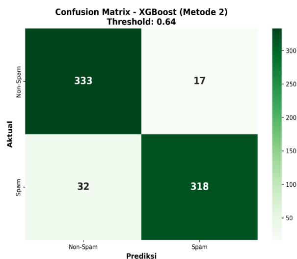
Gambar IV. 7 Confusion matrix XGBoost Metode 2
