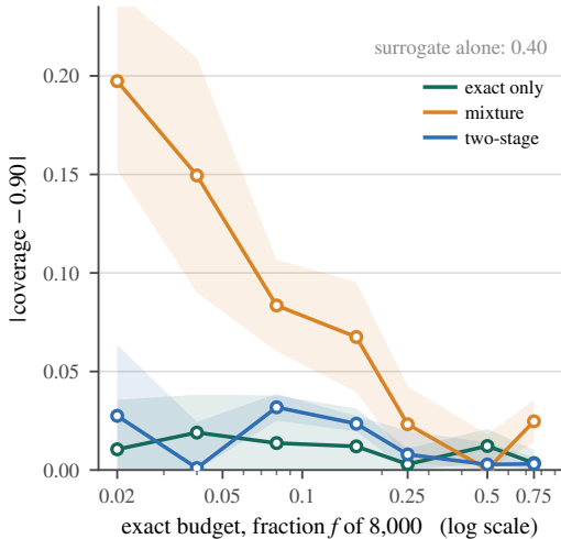
B Calibration vs. exact budget
