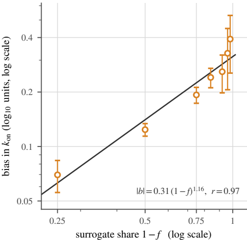
A Bias vs. surrogate share
