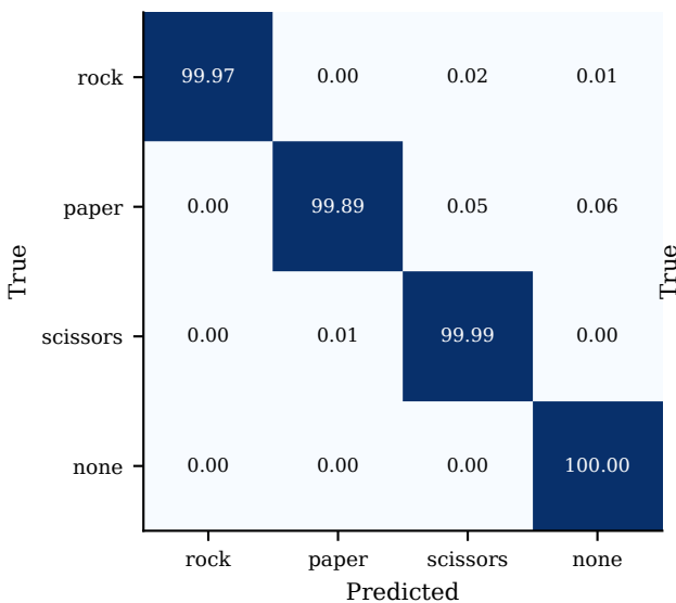
ResNet50 (n=5 folds)
