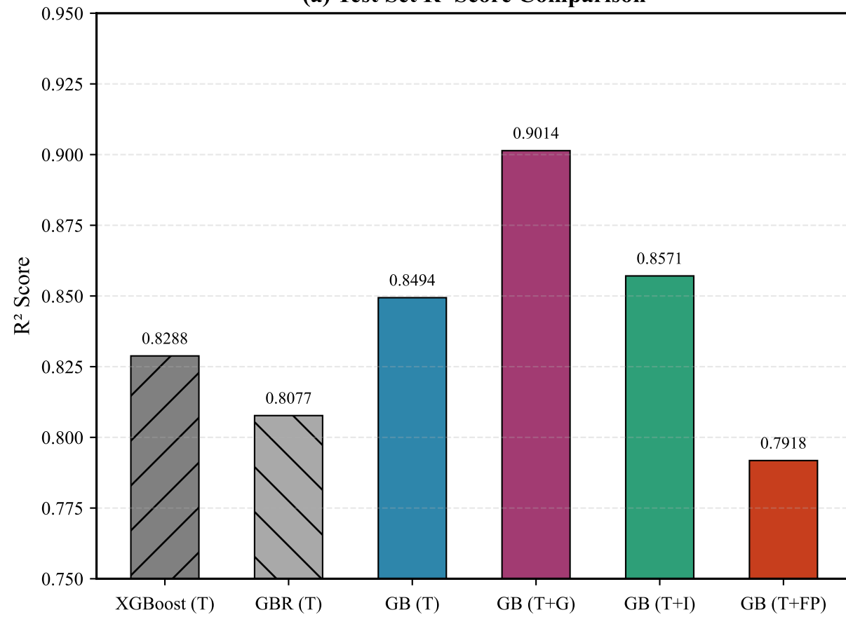
Performance Comparison: Traditional ML vs Gradient Boosting (Single/Multi-modal) (a) Test Set R 2 Score Comparison
