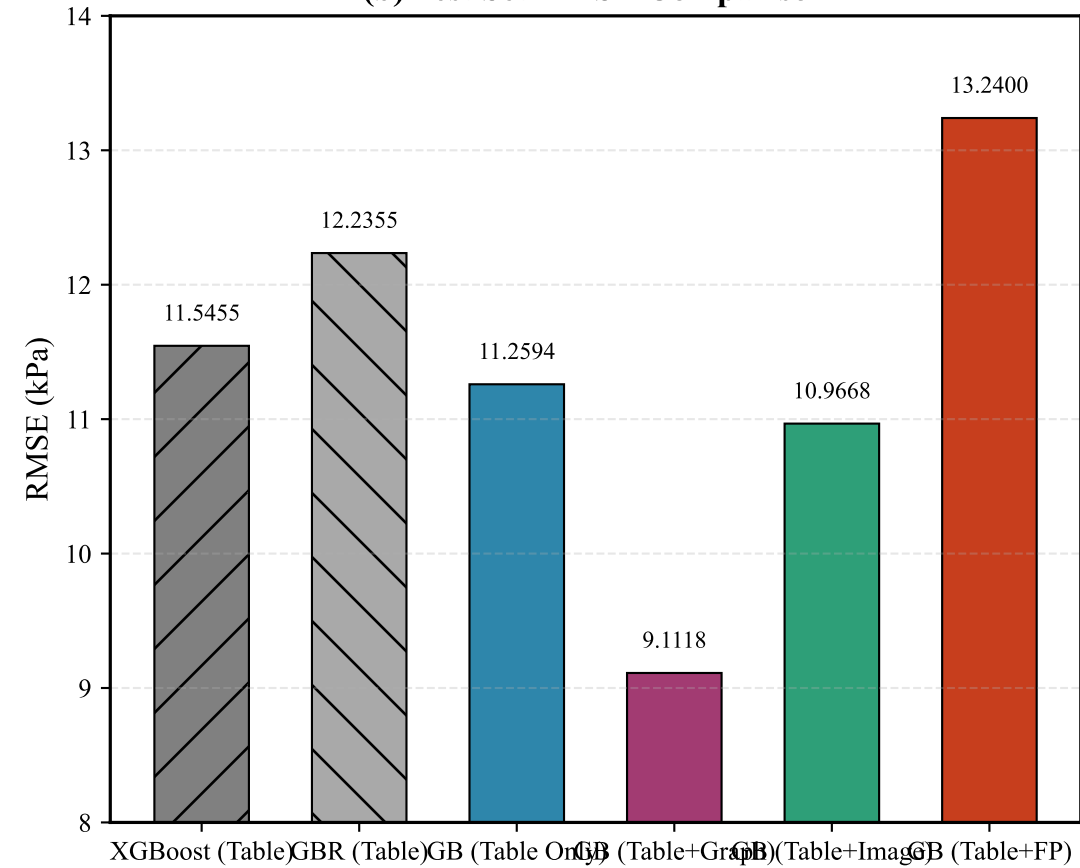
(b) Test Set RMSE Comparison
