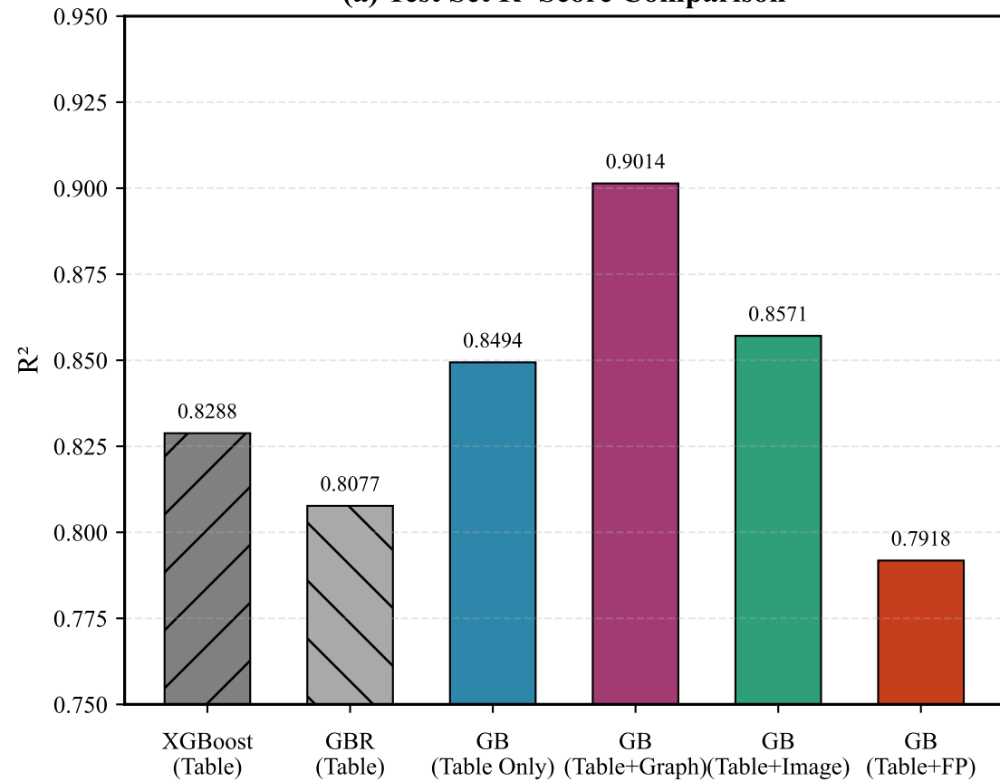
Performance Comparison: Traditional ML vs Gradient Boosting (Single/Multi-modal) (a) Test Set R 2 Score Comparison
