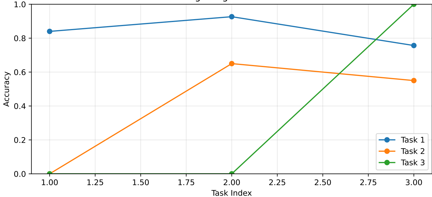
Forgetting Curve - M6
