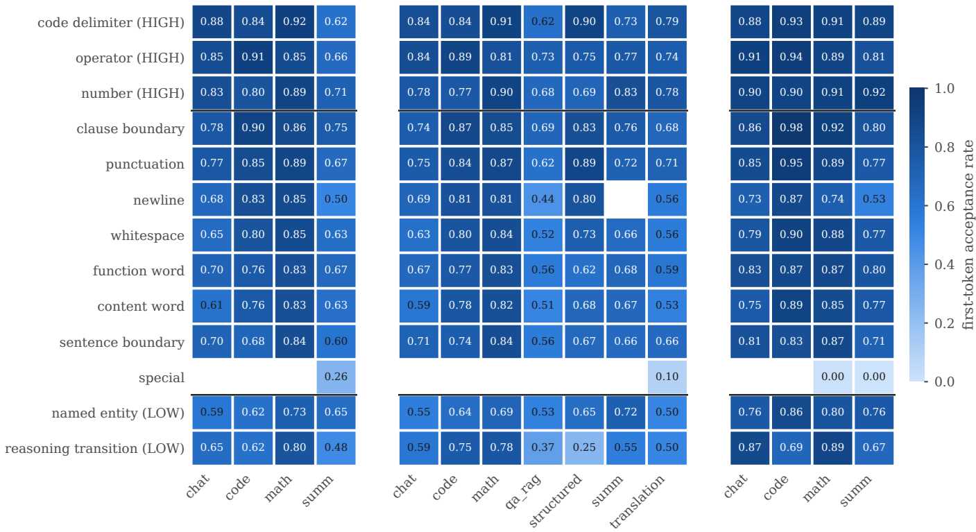
Qwen-v1 pooled HIGH 0.84 / LOW 0.65
