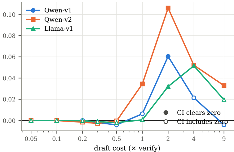
regret reduction
