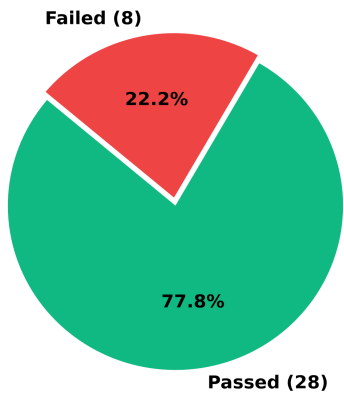
EduPathAI QA Test Case Outcomes (36 Total)
