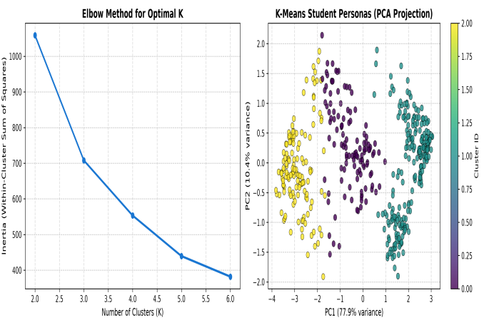
Figure 2: K-Means Behavioral Persona Clustering
