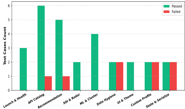
Test Execution Breakdown by Functional Category
