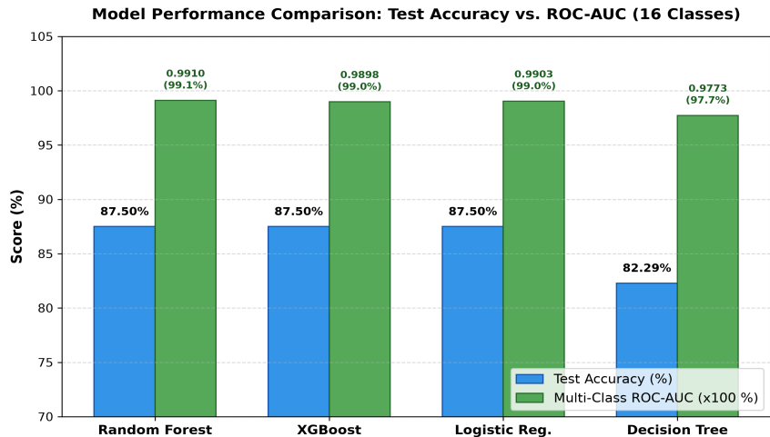
Figure 3: Accuracy vs ROC-AUC Generalization Benchmark Across Classifiers
